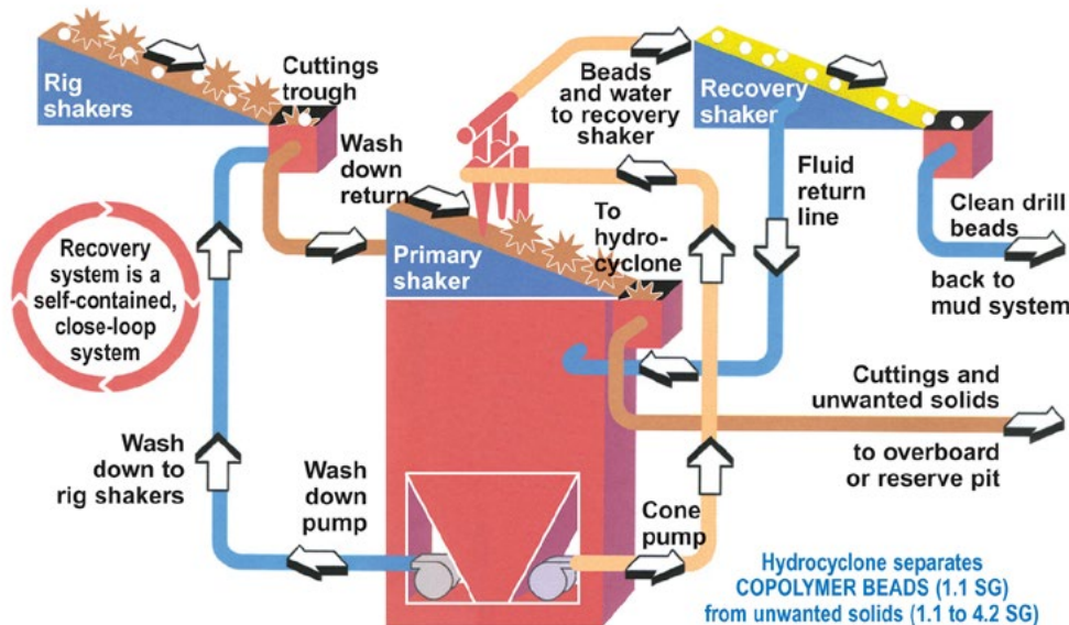
MMG Bead Recovery Unit Drill cuttings separation / bead recovery schematic
